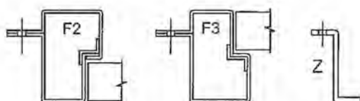
FLANGE MOUNTED FRAMES
